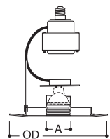
1479W White Trim with Black Baffle
